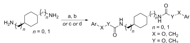
Scheme 1. Synthetic approaches to symmetric ISRIB analogues. Reagents and conditions: a) ClCH 2 C(O)Cl, DIEA, CH 2 Cl 2 ; b) ArOH, K 2 CO 3 , acetone; c) ArOCH 2 COOH, EDC, HOBT, DIEA, DMF or ArCH 2 OCOOH, HATU, DIEA, DMF; d) triphosgene, ArOH, DIEA, CH 2 Cl 2 .
