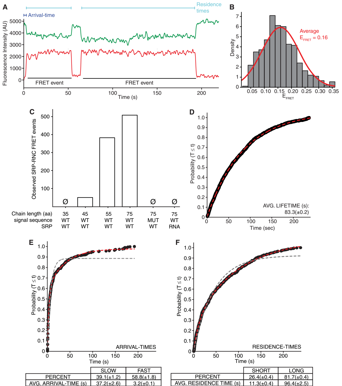
FIGURE 4. Nucleotide-labeled smFRET assay to detect SRP-RNC interactions. All results shown use the nucleotide-labeled assay. A , single-molecule trace of Cy5-labeled SRP delivered at time = 0 to slides with immobilized Cy3B-labeled 75-aa RNC visualized using TIRFM. The fluorescence intensity of the Cy3B (green) and Cy5 (red) signals is shown. FRET events, arrival time, and residence times are labeled. AU, arbitrary units. B , histogram plot with normal fit of observed E_{\text{FRET}} values when SRP was delivered to 75-aa RNC. For the experiment shown in this panel, the 50S subunits were unlabeled (see “Experimental Procedures”). C , bar plot of observed SRP-RNC FRET events and their dependence on aa length of nascent chains on stalled RNC, nature of the signal sequence (WT or mutant (MUT) (see “Experimental Procedures” for sequence)), and composition of SRP (WT or 4.5S RNA alone (RNA)). \emptyset indicates that no events were measured. D , cumulative distribution of lifetimes of the dye on SRP when SRP was directly immobilized on the slide surface. E and F , cumulative distributions of arrival times ( E ) and residence times ( F ) of SRP binding to 75-aa RNC. Gray and red lines indicate fits to single and double exponentials, respectively. The percentage and average (AVG; \pm 95% confidence interval of fit) arrival and residence times to the double exponential for each type of event are indicated ( n \geq 419 binding events).
